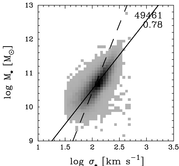
Figure 14. Mass-velocity dispersion relation for our sample. The solid line is a robust fit for the data while dashed one is a fitting assuming M_* \propto \sigma^4 .
