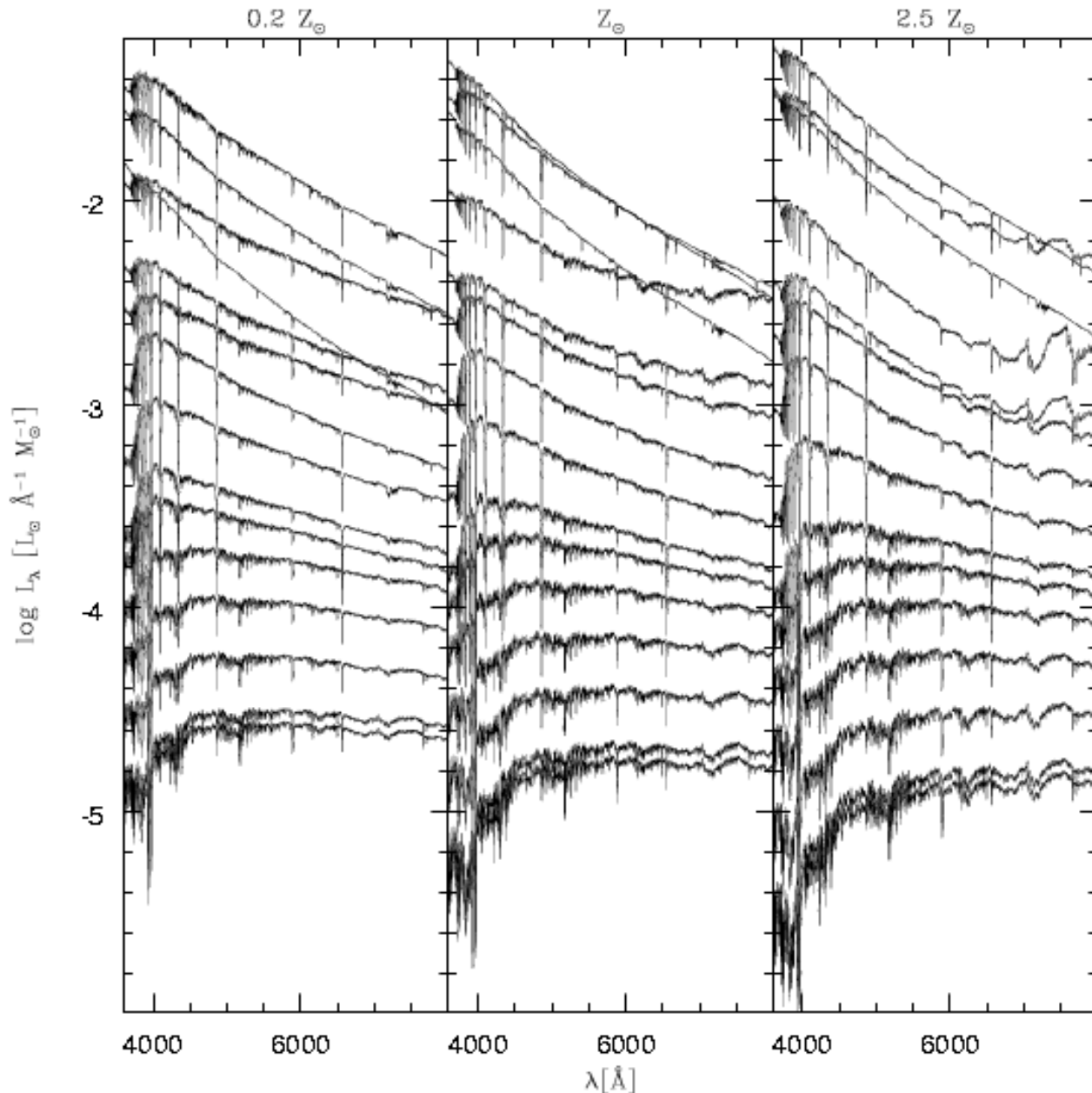
Figure 1. Spectra of the 45 SSPs used in the spectral synthesis (from BC03). The base comprises 3 different metallicities, Z = 0.2 , 1 and 2.5 Z_{\odot} , and 15 ages: From top to bottom, t = 0.001 , 0.00316, 0.00501, 0.01, 0.02512, 0.04, 0.10152, 0.28612, 0.64054, 0.90479, 1.434, 2.5, 5, 11 and 13 Gyr. All SSPs are normalized to 1 M_{\odot} at t = 0 .
