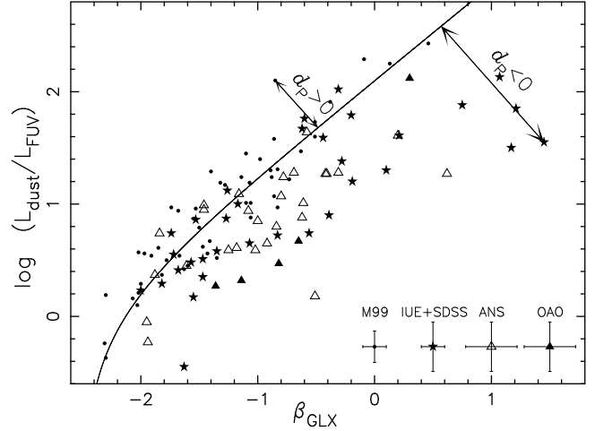
Figure 1. Ratio of far-infrared to ultraviolet luminosities plotted against ultraviolet spectral slope (the ‘IRX-UV diagram’). The data points are from the sample compiled in Section 2.1 (median measurement errors for each subsample are indicated in the lower right corner). The solid line shows the mean IRX-UV relation for the 50 starburst galaxies in this sample (equation 2).
