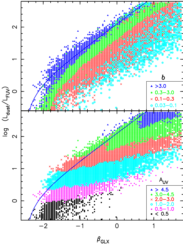
Figure 4. Ratio of far-infrared to ultraviolet luminosities plotted against ultraviolet spectral slope (the ‘IRX-UV diagram’) for the model library described in Section 4. Upper panel: the IRX-UV plane has been binned and coded to reflect the average ratio of present to past-averaged star formation rates of the galaxies that fall into each bin. Lower panel: the IRX-UV plane has been binned and coded to reflect the average ultraviolet attenuation A_{\text{FUV}} of the galaxies that fall into each bin. In each panel, the solid line shows the mean starburst IRX-UV relation from Fig. 1.
