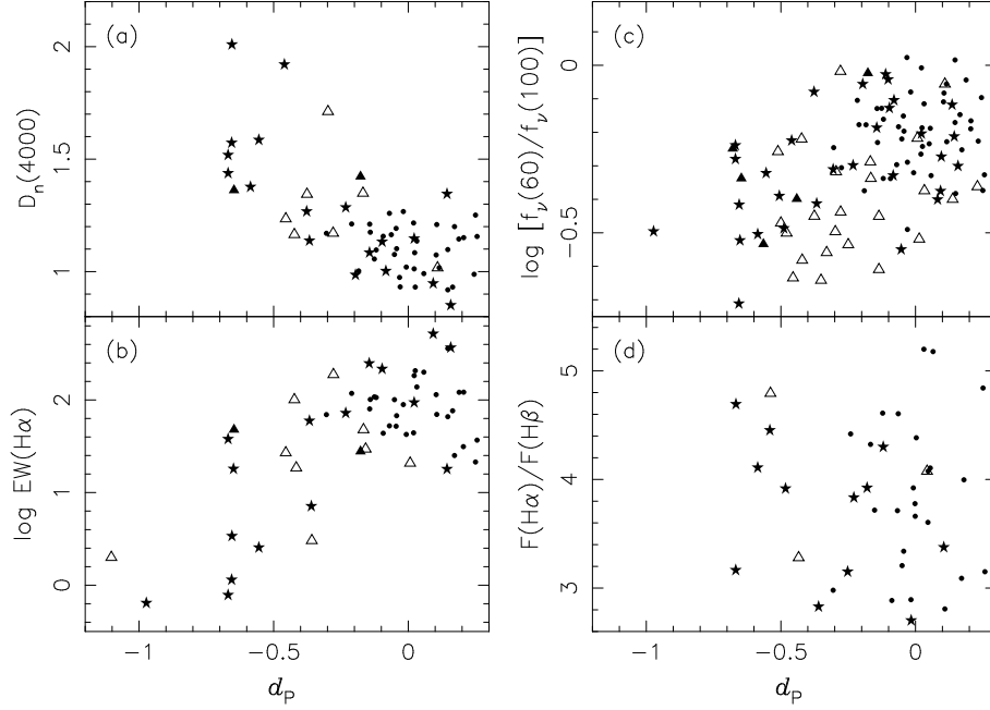
Figure 2. (a) spectral discontinuity at 4000 Å, (b) H \alpha emission equivalent width, (c) ratio of IRAS f_\nu (60 \mu m) and f_\nu (100 \mu m) flux densities and (d) H \alpha /H \beta ratio plotted as a function of perpendicular distance from the mean starburst IRX-UV relation, for the subsets of galaxies for which these observed quantities are available in the sample of Fig. 1. The different symbols have the same meaning as in Fig. 1.
