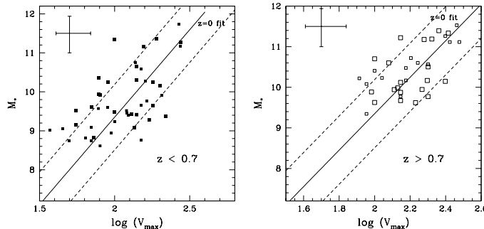
Figure 2. The stellar mass Tully-Fisher relationship ( M_* vs. V_{\max} ). The solid and dashed lines are the z = 0 relationship found by Bell & de Jong (2001) for nearly disks and its \pm 3 \sigma scatter. The error bar is the average error with large points having errors lower than this average, with smaller points having errors larger than the average.
