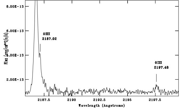
Fig. 12. Two "new" Bowen lines from the primary decay (40.85 eV). The \lambda 2187.02 line falls on the wings of the He II Fowler line \lambda 2186.60, while the \lambda 2197.48 line is weak but unblended. All wavelengths are in air.
