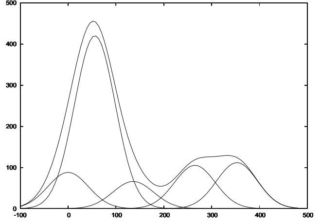
Fig. 15. The five O III resonance lines close to \lambda 374, with relative height proportional to their intensity, and \text{FWHM} = 100 \text{ km s}^{-1} . The upper line represents the sum of the five components. The x-axis gives the line separation in \text{km s}^{-1} , with zero-point at \lambda 374.00.
