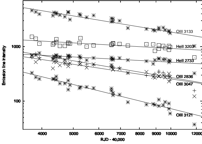
Fig. 11. A log-log plot of the decrease with time of the ELI of the He II and O III lines from 1978 to 1995 in IUE spectra. The last data are from STIS (Oct.10, 2000). The ELI are in units of 10^{-13} erg cm ^{-2} s ^{-1} . The power-law fits to the data (straight lines) have indices \sim -0.33 , \sim -0.97 , and \sim -1.48 , for the two He II lines ( \lambda 2733 and \lambda 3203), the three O III O1 lines ( \lambda 2836, \lambda 3047 and \lambda 3132), and the O III O3 line ( \lambda 3122), respectively.
