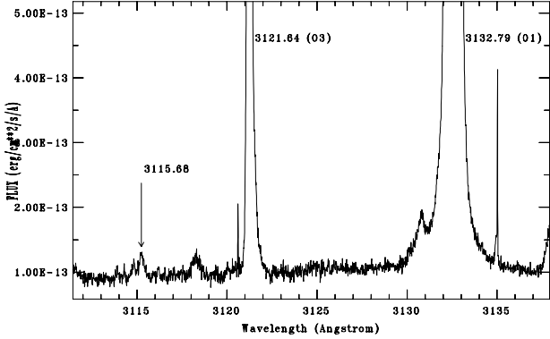
Fig. 8. The UVES spectrum shows the strongest line of each of the three Bowen excitation channels. From left to right: the very weak \lambda 3115.68 line (from 2p3d\ ^3P_0 , at -250\text{ km s}^{-1} from He II Ly- \alpha ), the O3 \lambda 3121.64 line (from 2p3d\ ^3P_1 , at -88.2\text{ km s}^{-1} from He II Ly- \alpha ), and the strong O1 \lambda 3132.79 line (from 2p3d\ ^3P_2 , at +16.4\text{ km s}^{-1} from He II Ly- \alpha ).
