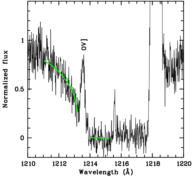
Fig. 5. The interstellar Ly \alpha line. Our best fit to the damping wing, excluding the [O V] \lambda 1213.81 emission line, implies a hydrogen column density N(\text{H})=6.9 \times 10^{19} \text{ cm}^{-2} and is shown as a solid line.
