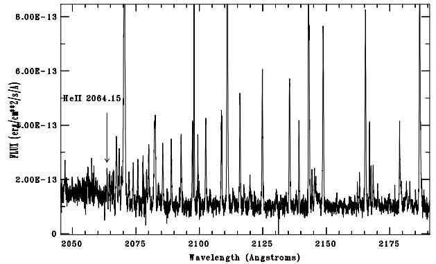
Fig. 1. The He II Fowler lines near the head of the ( n-3 ) series. The last resolved line is ( 37 \rightarrow 3 ) \lambda 2063.49.
