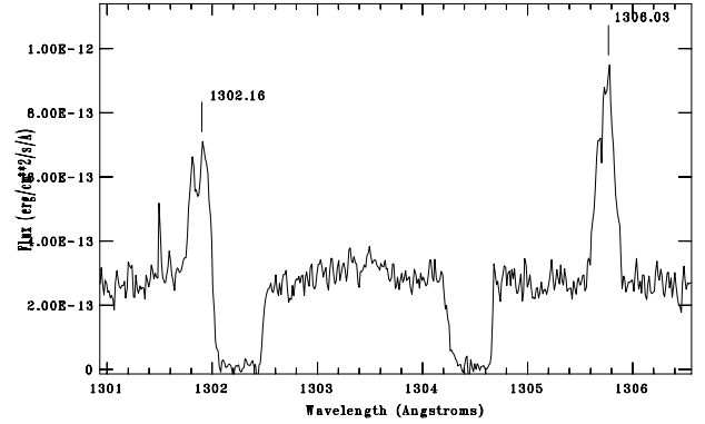
Fig. 16. The resonance O I lines close to \lambda 1304. The two absorption features are IS and due to the zero-volt lines of O I \lambda 1302.16 and Si II \lambda 1304.37. This latter line has fully absorbed the O I \lambda 1304.86 line.
