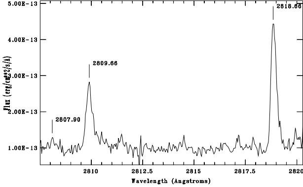
Fig. 7. The weak O III Bowen lines near \lambda 2800 in STIS
