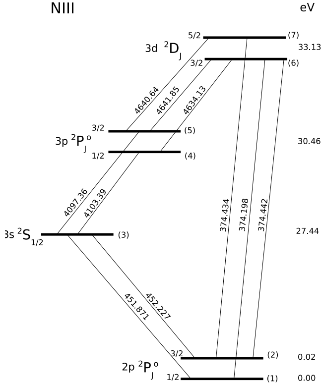
Fig. 13. A partial Grotrian diagram for N III. Levels are identified by a number index 1-7 to facilitate reading the text.
