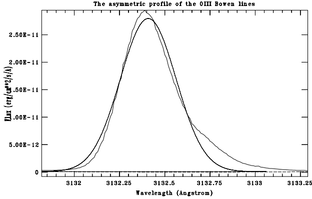
Fig. 10. The asymmetric profile of the O III \lambda 3133 line and a gaussian fit with FWHM=34.5 km s -1 . The same kind of profile is present also in other lines, see sect. 4.3.
