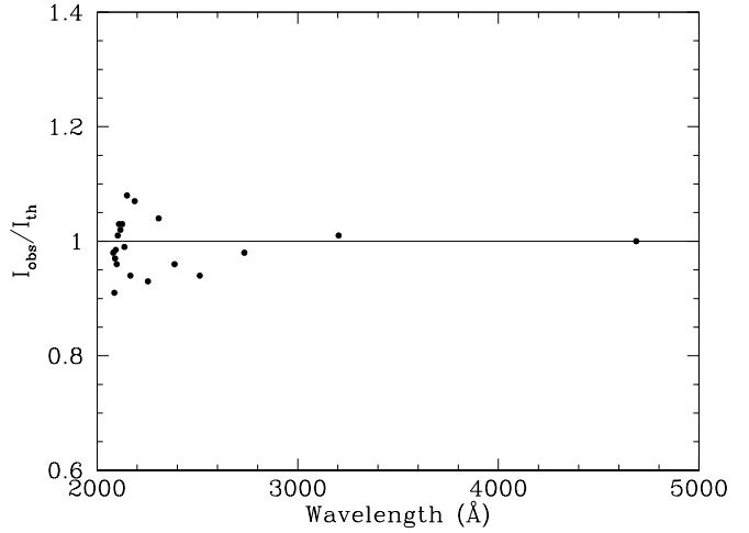
Fig. 2. The I_{\text{obs}}/I_{\text{th}} ratio relative to I_{4686} for the He II Fowler lines listed in Table 2.
